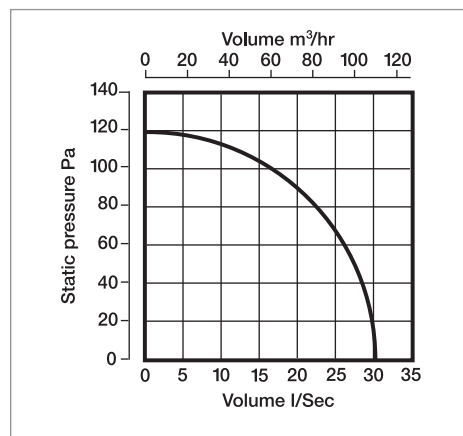
Performance - CF200
