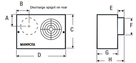
Dimensions - CF200
