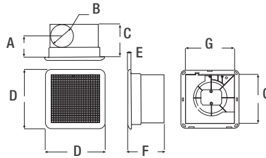
Dimensions - Multi-Vent (Flush Fitting)
