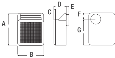
Dimensions - Multi-Vent (Surface Mount)
