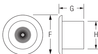
Diffuser
