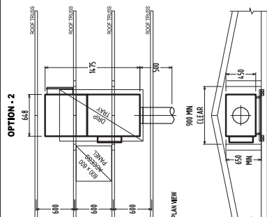
SIDE VIEW IN-CEILING MOUNTING AIR SMART FAN COIL UNIT
