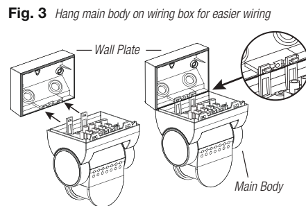
Fig. 3 Hang main body on wiring box for easier wiring
