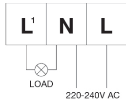
Wiring Diagram
